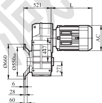
GFAF/GFHF157
