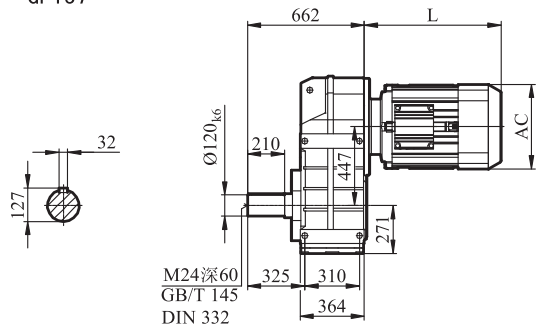
GFA/GFH157
